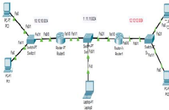
Gambar 4. Design Jaringan
