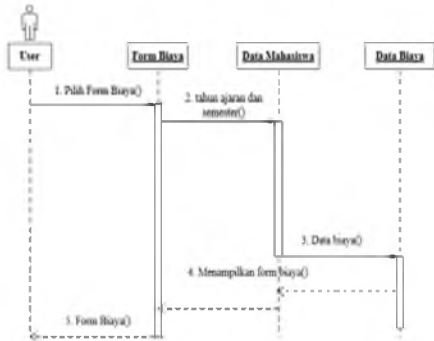
Gambar 5. Sequence diagram lihat data biaya
